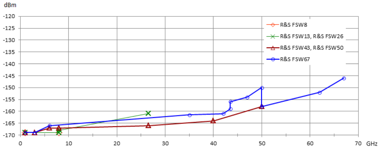
Typical displayed average noise level of the R&S®FSW models for f > 1 GHz with RF preamplifier option R&S®FSW-B24 5 , preamplifier gain = 30 dB.
